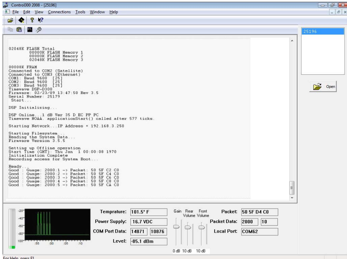
Figure 5: DSP-D300 Control300 Start Screen
