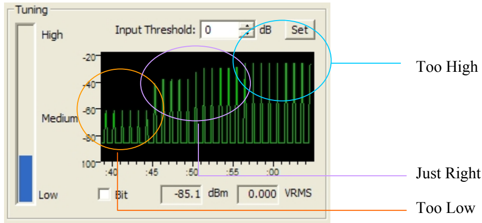
Figure 8: Control300/DSP-D300 Input Threshold
