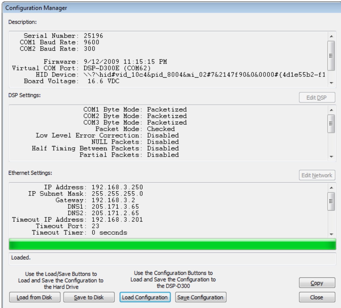
Figure 6: Control300 Configuration Manager
