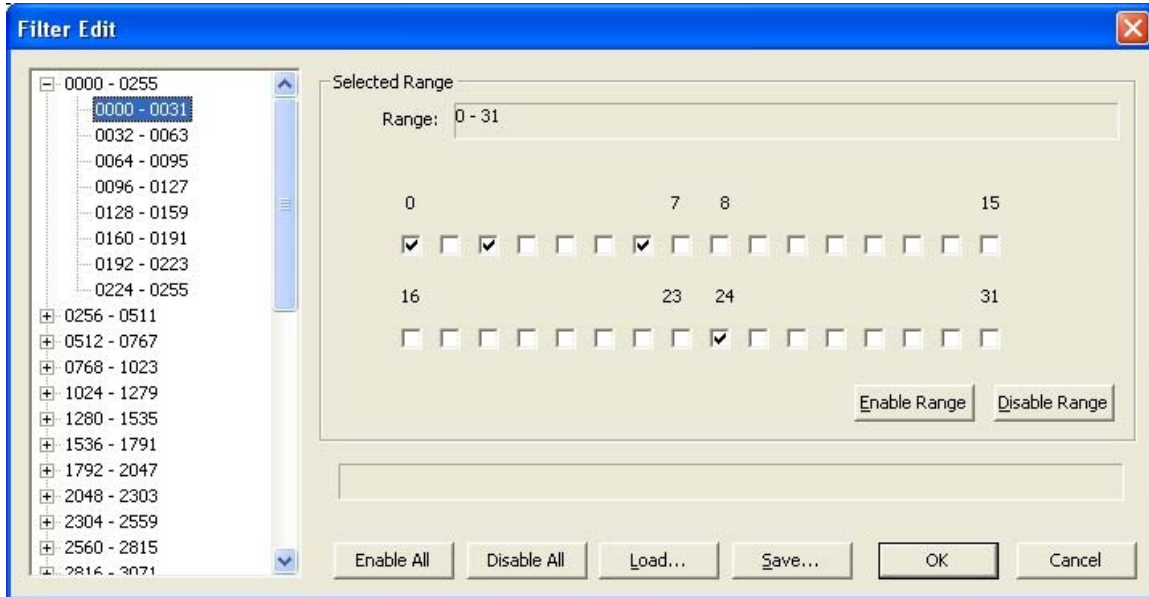
Figure 15: DSP-D300 Control300 Filter Editor
