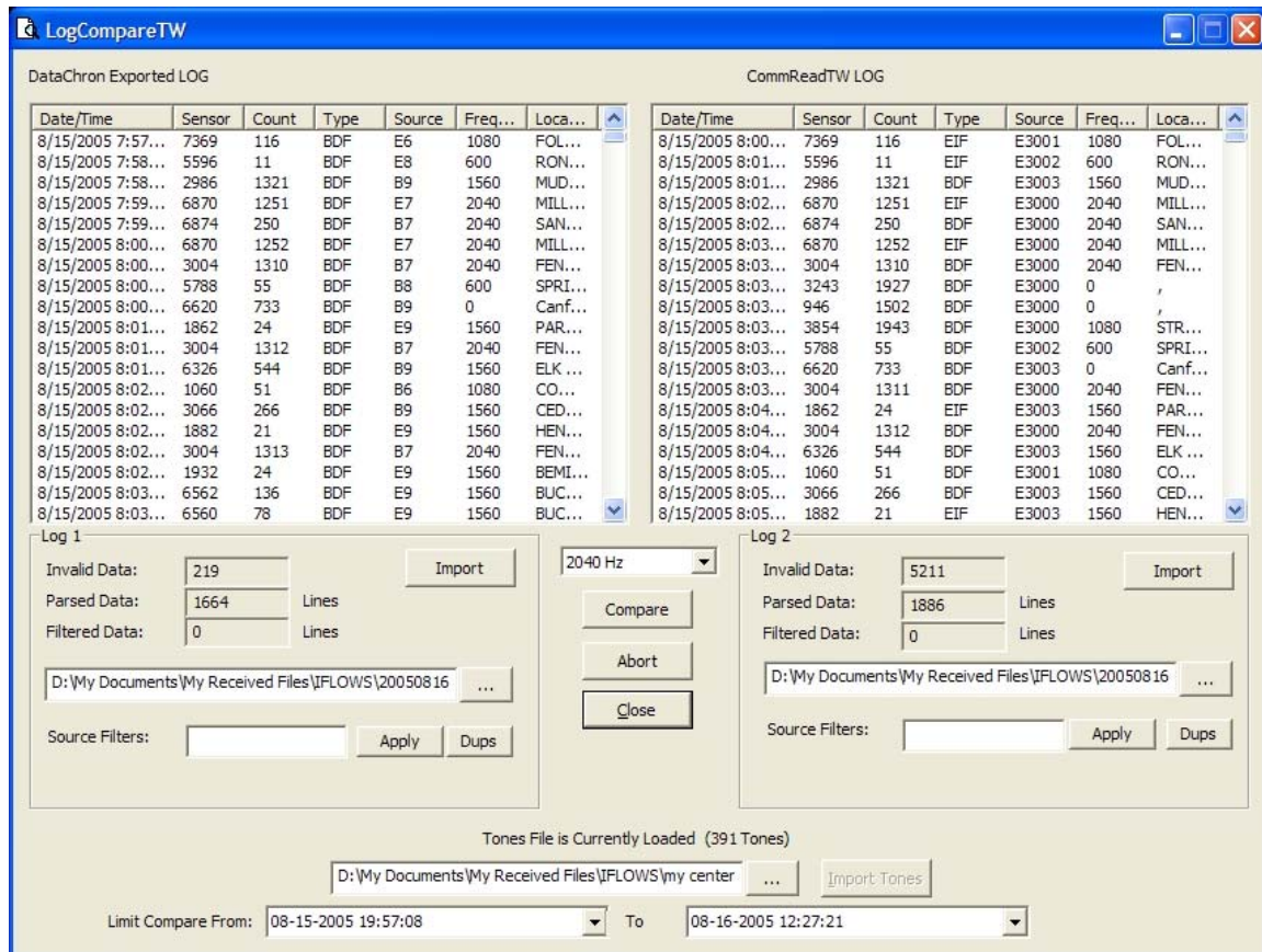
Figure 26: DSP-D300 LogCompareTW Screen
