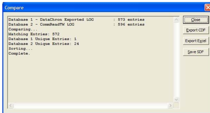
Figure 27: DSP-D300 LogCompareTW Compare Screen
