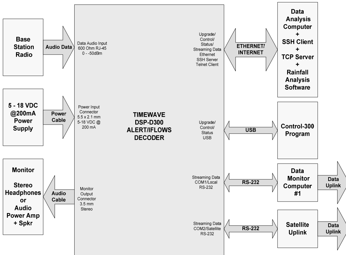
Figure 29: DSP-D300 Installation Block Diagram
