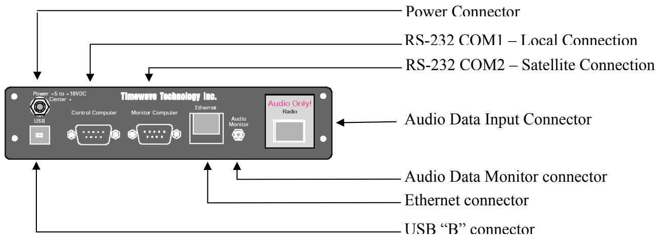
Figure 28: DSP-D300 Back Panel
