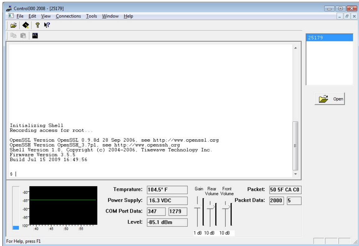
Figure 7: DSP-D300 Control300 Shell Screen
