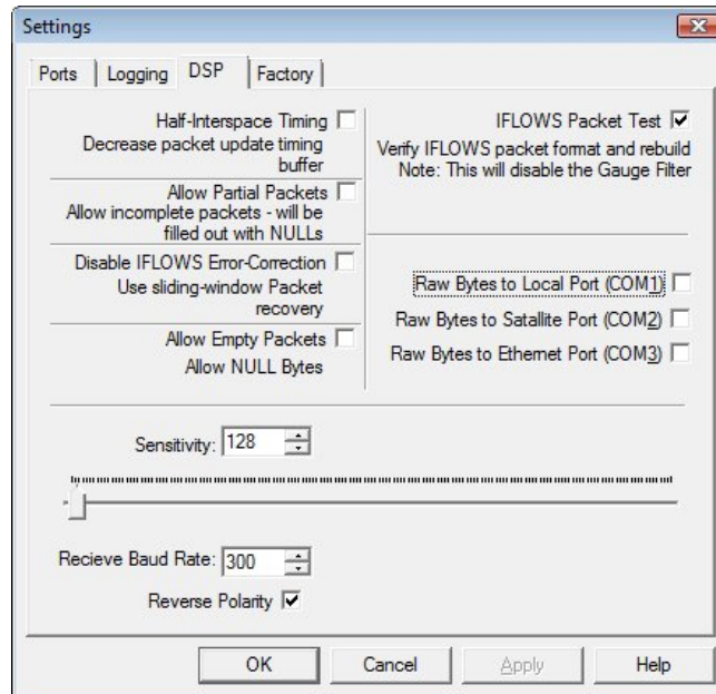
Figure 16: DSP-D300 Control300 DSP Settings
